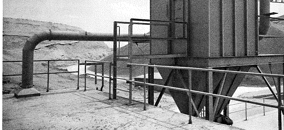
Wheelabrator Ultra-Filtration Unit providing dust-free air to control room.
